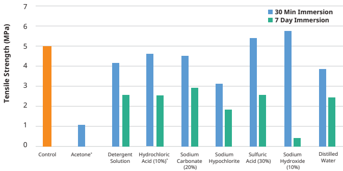
FIGURE 4 RUBBER-65A BLK
